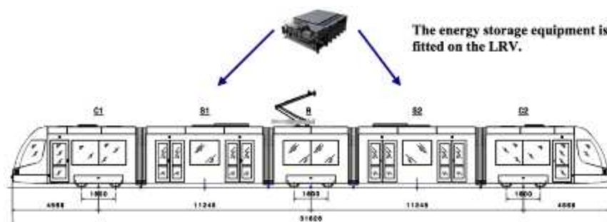
The energy storage modules are fitted on the train connected in parallel with the pantograph.
