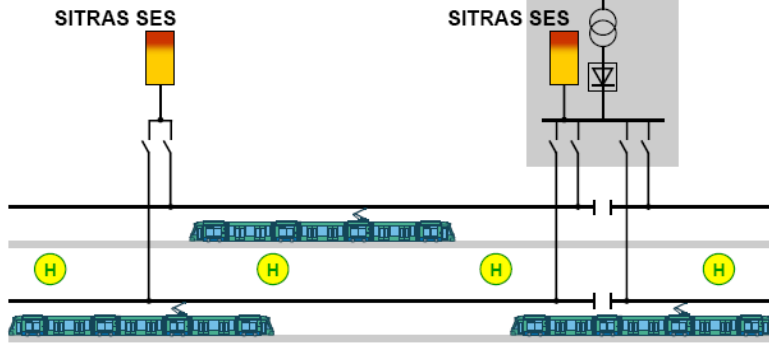
SITRAS SES at the line
